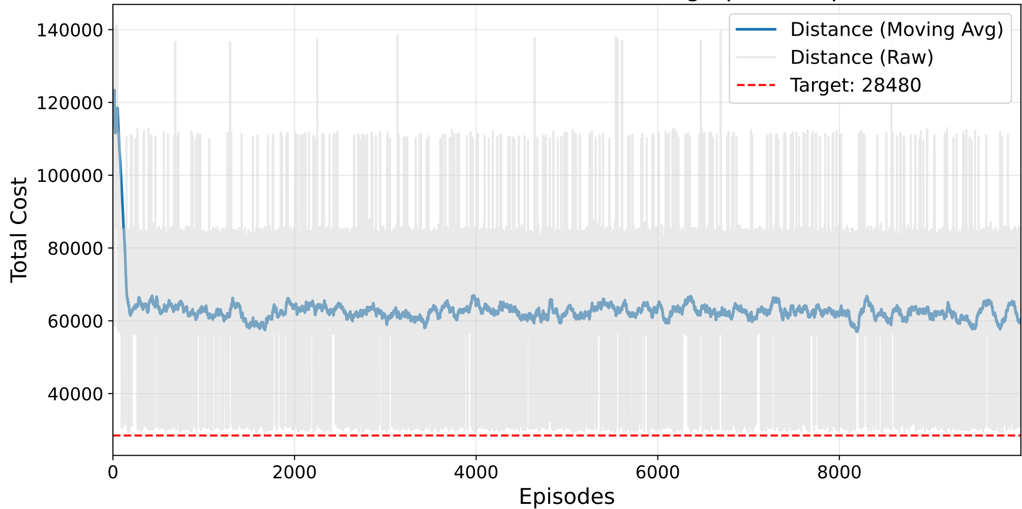
Final Masked AutoRL-SOP Training - p43.2.sop
